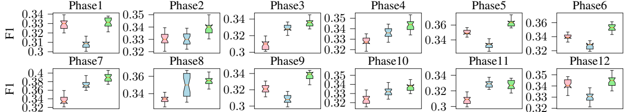
Fig. 7: Distribution of F1 scores with confidence intervals of the state-of-the-art model HATS (left, red), our proposed models HGCN (middle, blue) and STHGCN (right, green) over 10 different runs. Notched box plots best viewed in color.
